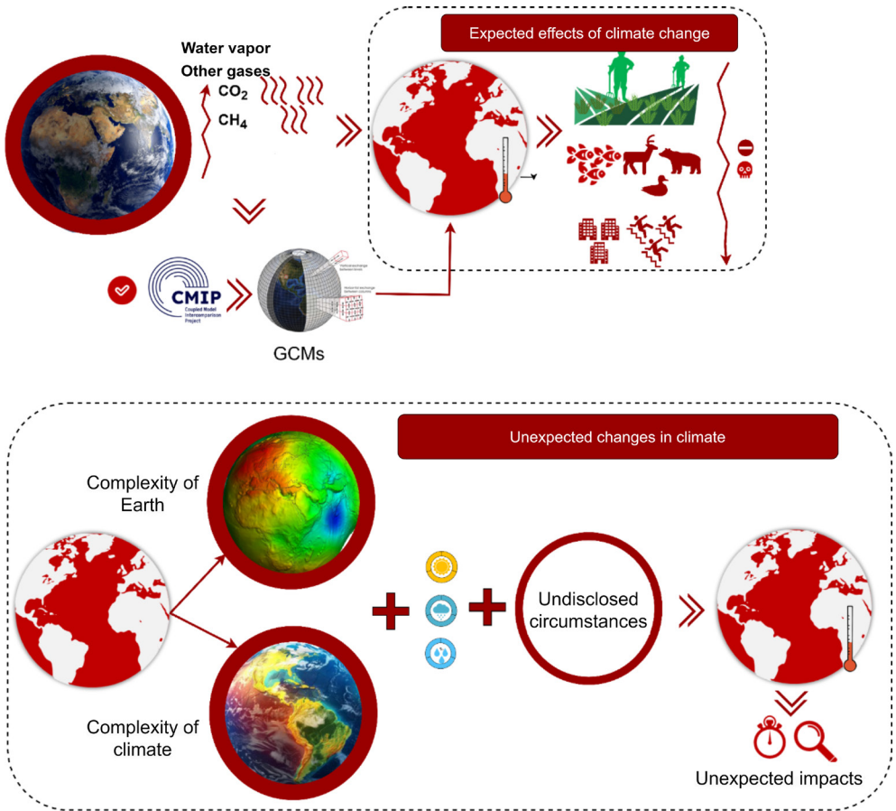
Fig. 11. Expected and unexpected impacts of climate change
