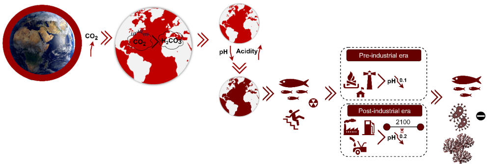
Fig. 9. Impacts of rising ocean acidity on global climate change
